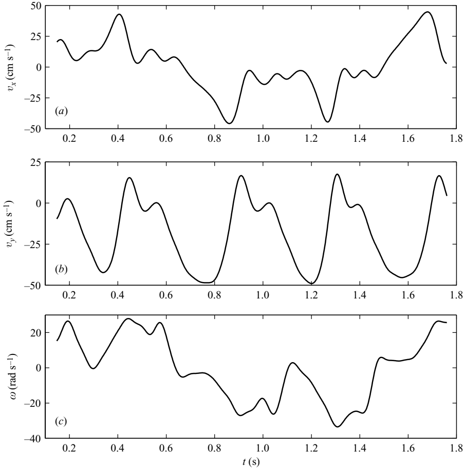
FIGURE 6. Measured velocities as functions of time for the plate with h=0.162 cm and \beta=1/6 displaying irregular motion, see trajectory (1) in figure 2(b). (a) The horizontal velocity component, (b) the vertical velocity component, and (c) the angular velocity. The irregular motion involves long gliding segments at low angle of attack with descent velocities up to v_y = -50 cm s -1 followed by centre-of-mass elevation with upward velocities up to v_y = 20 cm s -1 .
