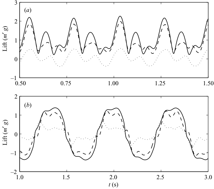
FIGURE 16. Measured (solid line), translational (dotted line), and rotational lift (dashed line): (a) tumbling with \beta = 1/5 and (b) fluttering with \beta = 1/14 . In (a) the average value of the translational lift is small and its functional form is markedly different from the measured lift, whereas the rotational lift captures the main features of the measurements. In (b) both translational and rotational lift have significant contributions and the functional forms are similar.
