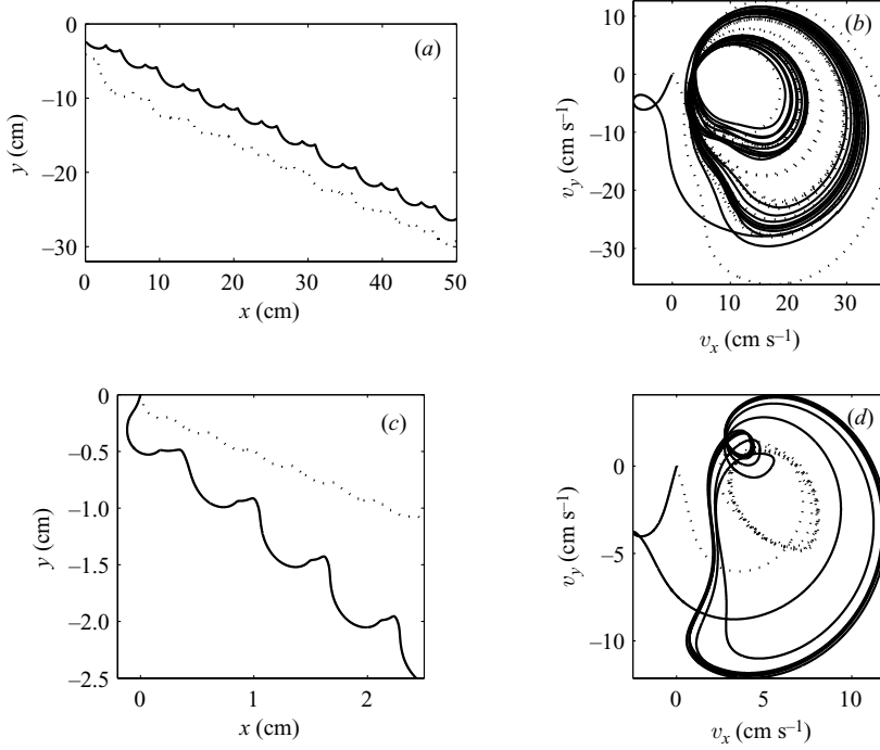
FIGURE 8. Periodic solutions and dependence on initial conditions investigated using direct numerical simulations: (a) trajectory and (b) v_x versus v_y for a tumbling plate with \beta=1/8 , Re=1025 , and I^*=0.17 with initial condition I (solid line) and II (dotted line) from table 2; (c) trajectory and (d) v_x versus v_y for a tumbling plate with \beta=1/4 , Re=10^2 , and I^*=0.36 with initial condition VI (solid line) and VII (dotted line) from table 2.
